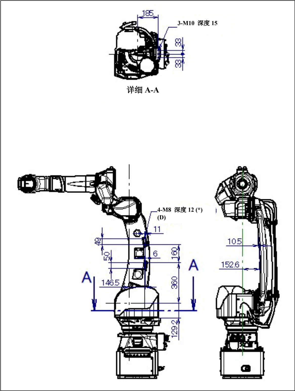
图 4.2 (c) 设备安装面尺寸 (2/2) (D 部+J2 机座部)
