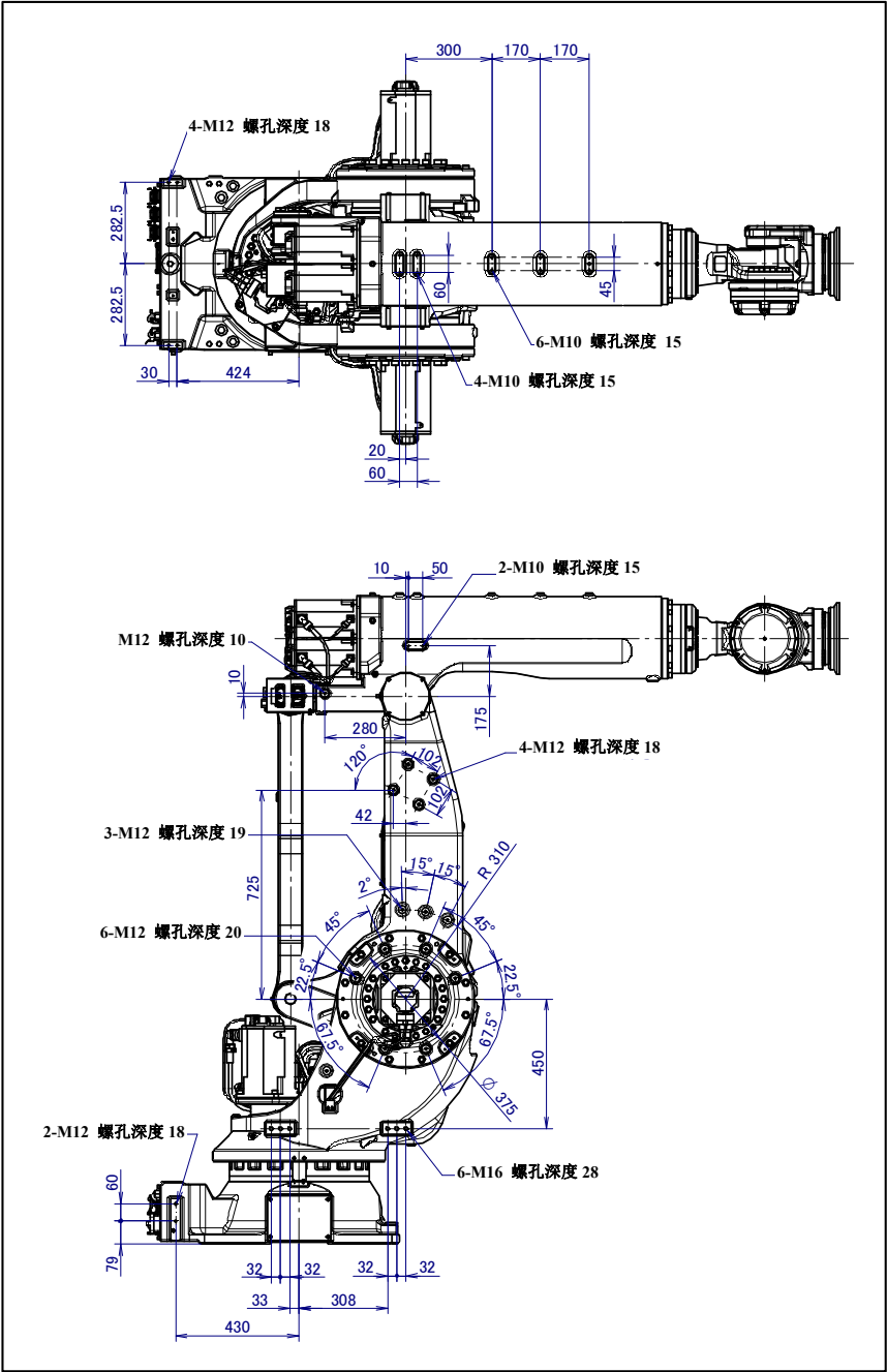
图 4.2 (e) 设备安装面尺寸 (M-900iB/280 (1/2))
