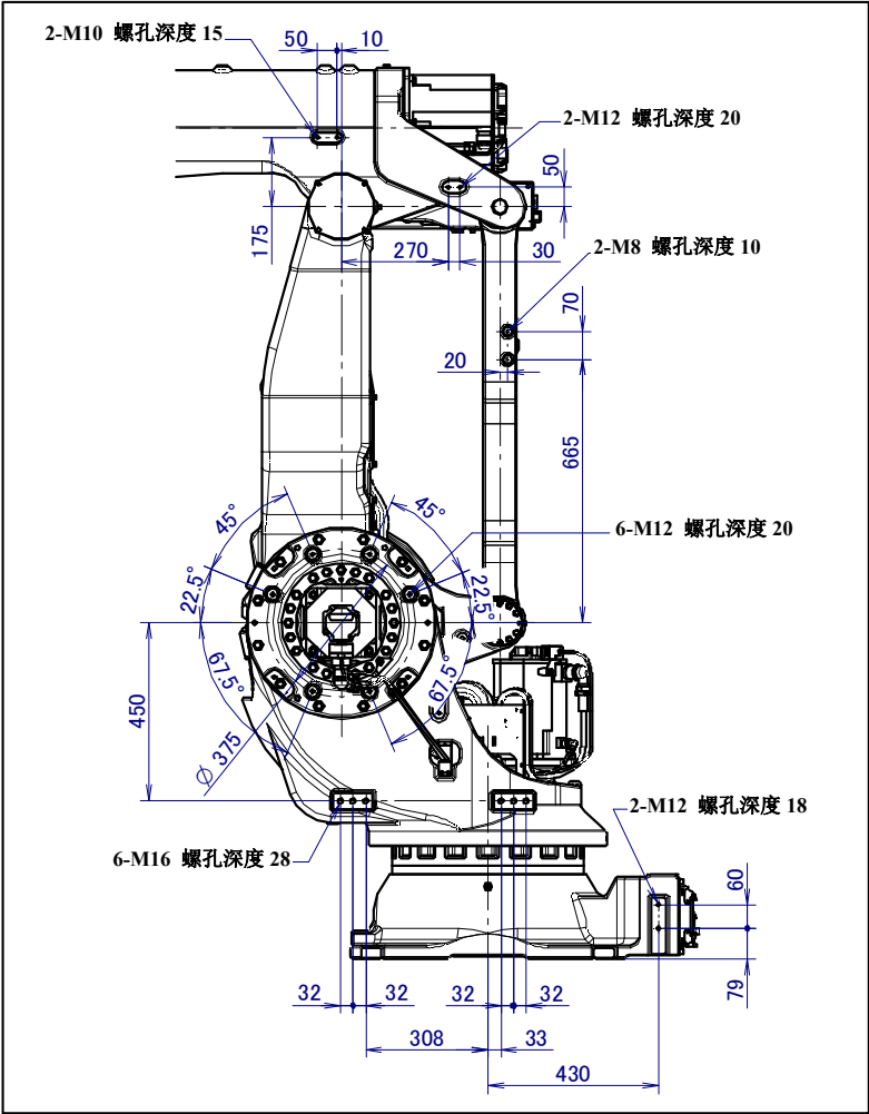
图 4.2 (f) 设备安装面尺寸 (M-900iB/280 (2/2))
