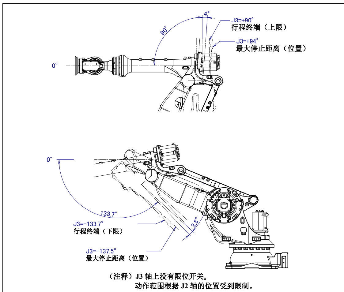
图 3.3 (e) J3 轴可动范围(M-900iB/360/280L/280)
