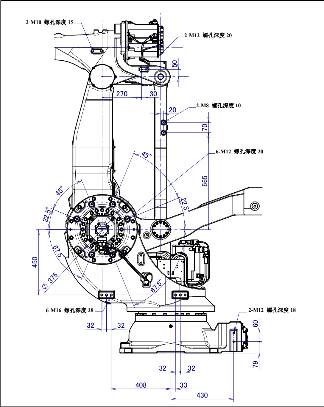
图 4.2 (h) 设备安装面尺寸 (M-900iB/330L (2/2))
