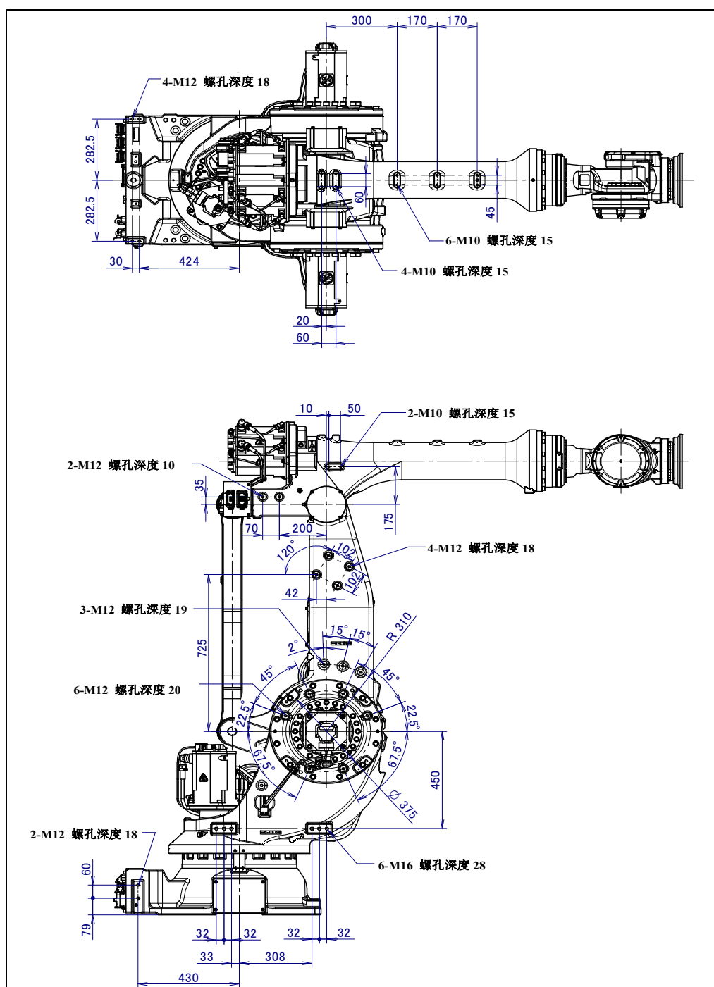
图 4.2 (a) 设备安装面尺寸 (M-900iB/360 (1/2))
