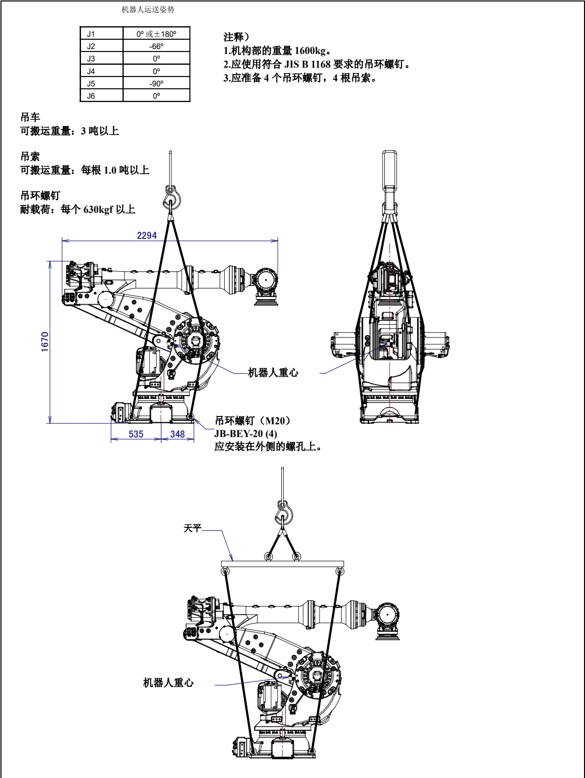
图 1.1 (c) 采用吊车搬运 (M-900iB/280L)
