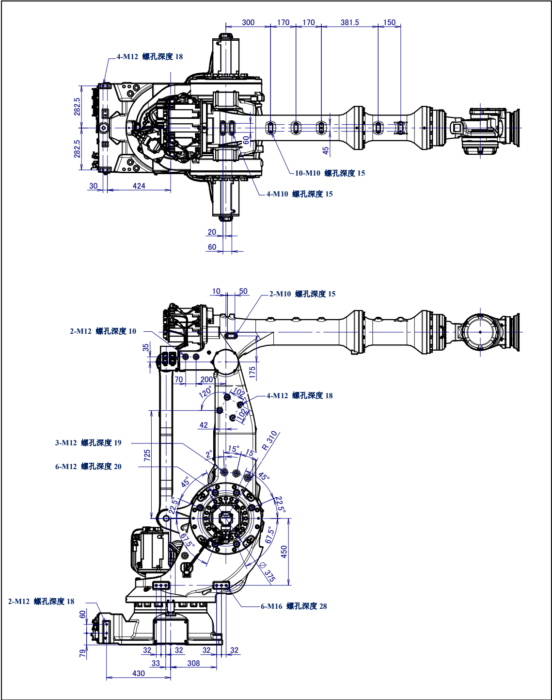
图 4.2 (c) 设备安装面尺寸 (M-900iB/280L (1/2))
