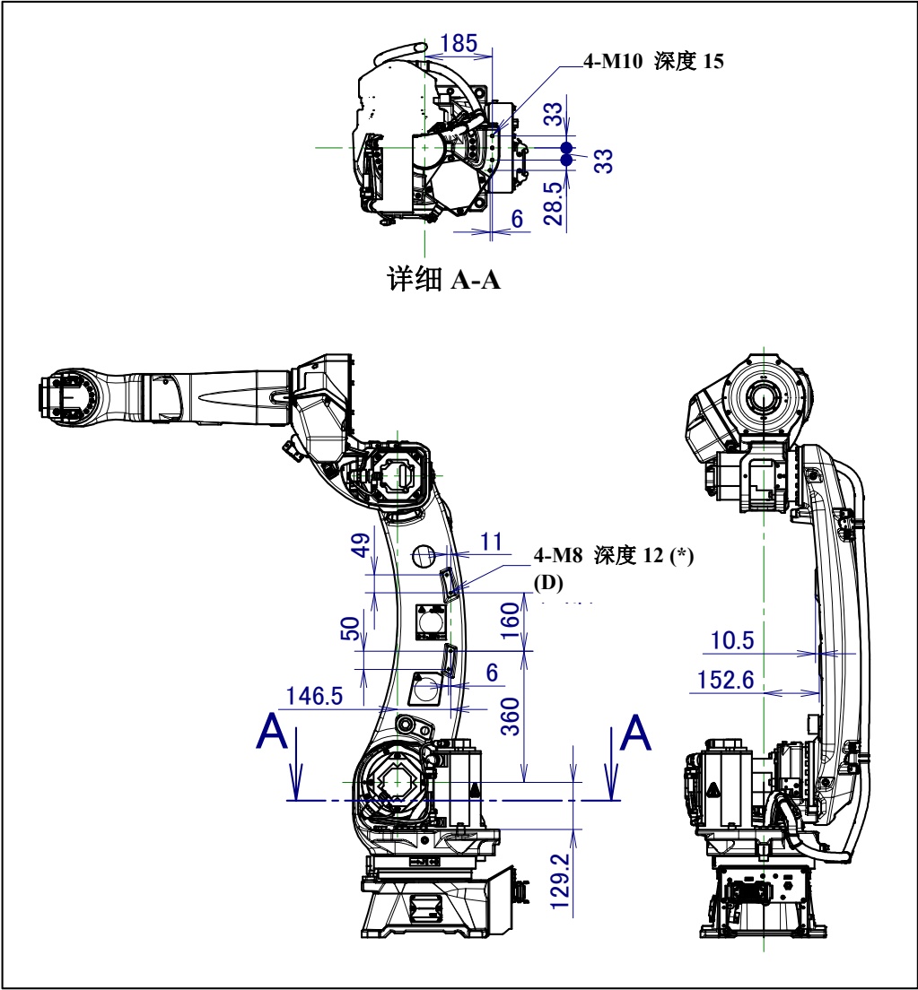
图 4.2 (c) 设备安装面尺寸 (2/2) (D 部+J2 机座部)
