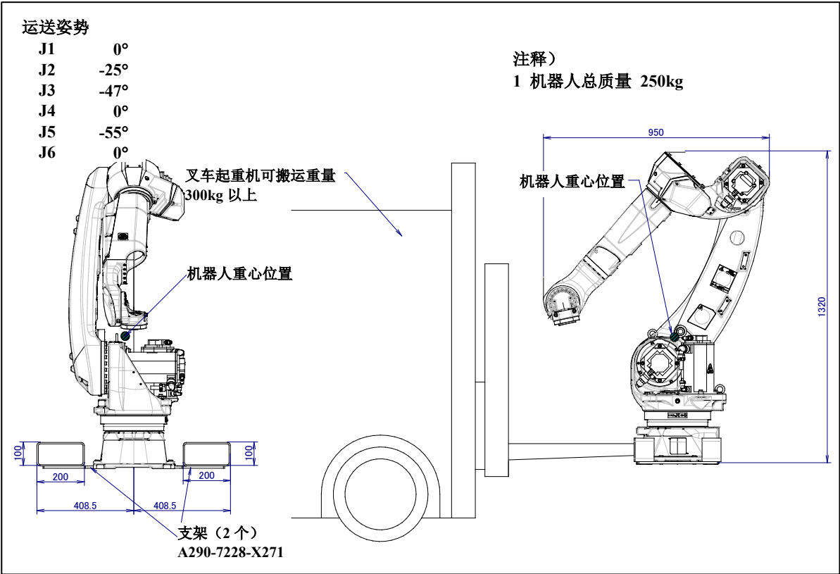
图 1.1 (c) 用叉车起重机搬运 (ARC Mate 120iD, ARC Mate 120iD/35, M-20iD/25/35)
