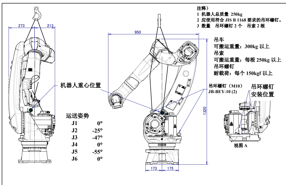
图 1.1 (a) 用吊车搬运 (ARC Mate 120iD, ARC Mate 120iD/35, M-20iD/25/35)
