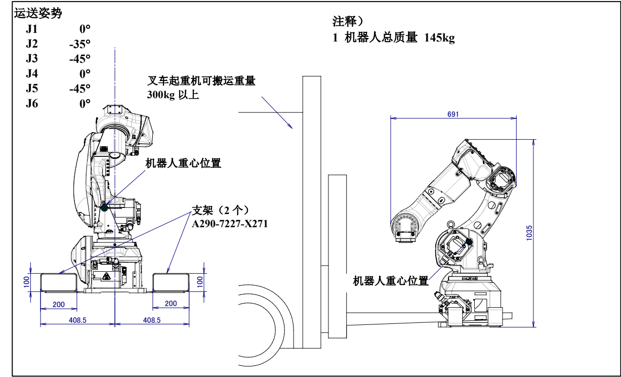
图 1.1 (h) 用叉车起重机搬运 (ARC Mate 100iD/16S, M-10iD/16S)
