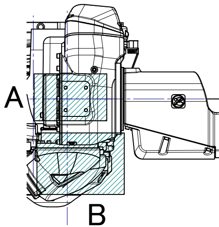
图 4.2 (c) 负载条件 (ARC Mate 100iD/16S, M-10iD/16S)
