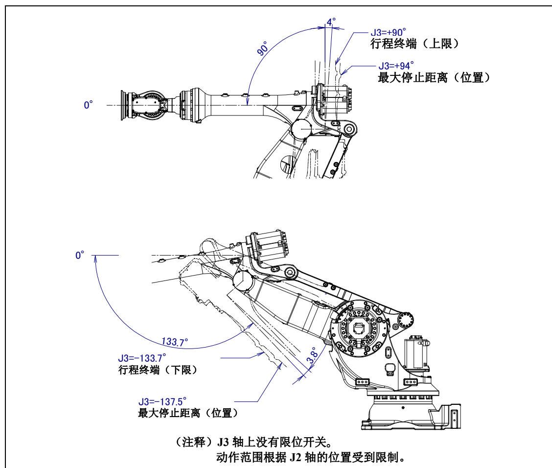
图 3.3 (e) J3 轴可动范围(M-900iB/360/360E/280L/280)
