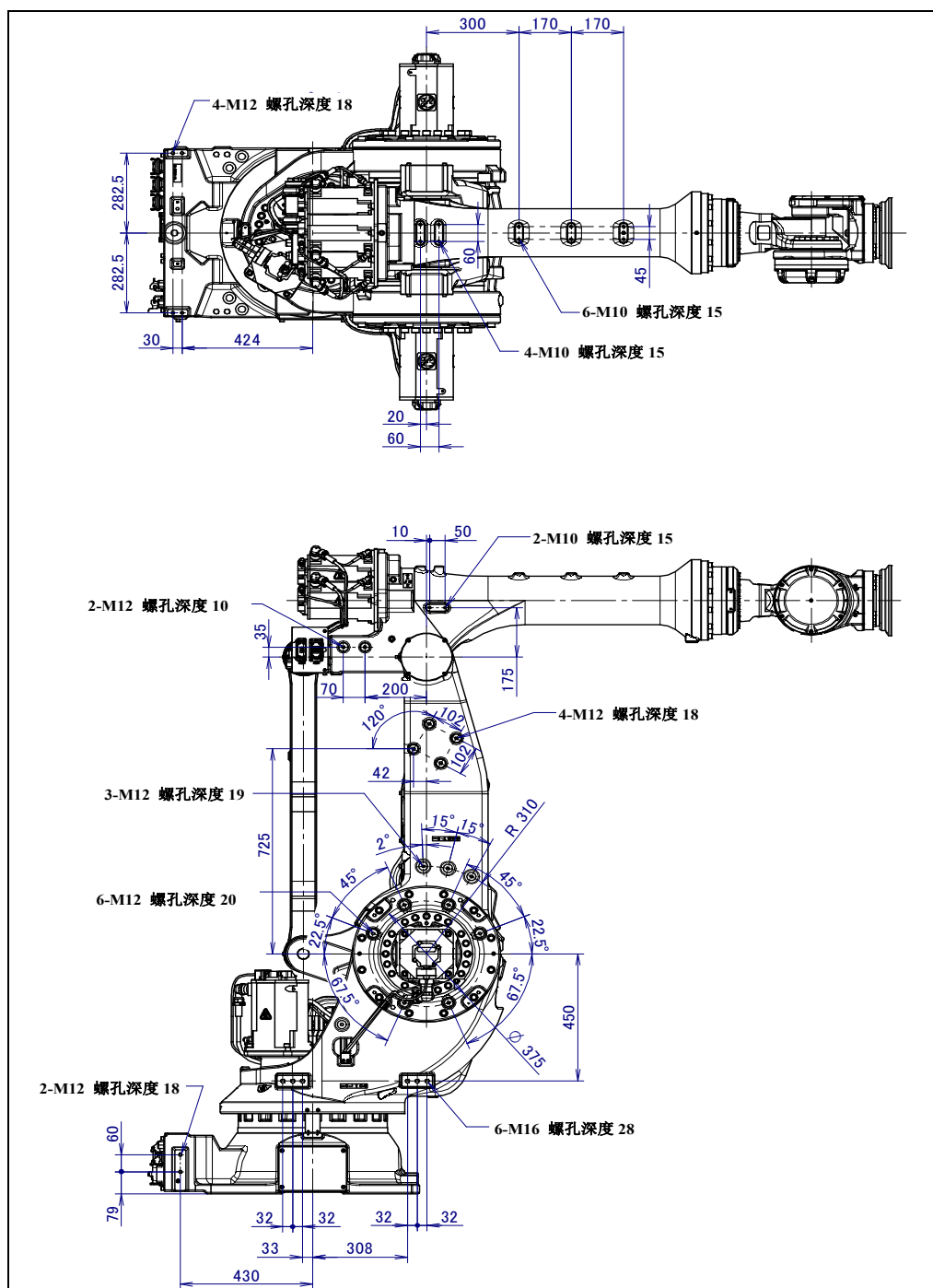
图 4.2 (a) 设备安装面尺寸 (M-900iB/360/360E (1/2))
