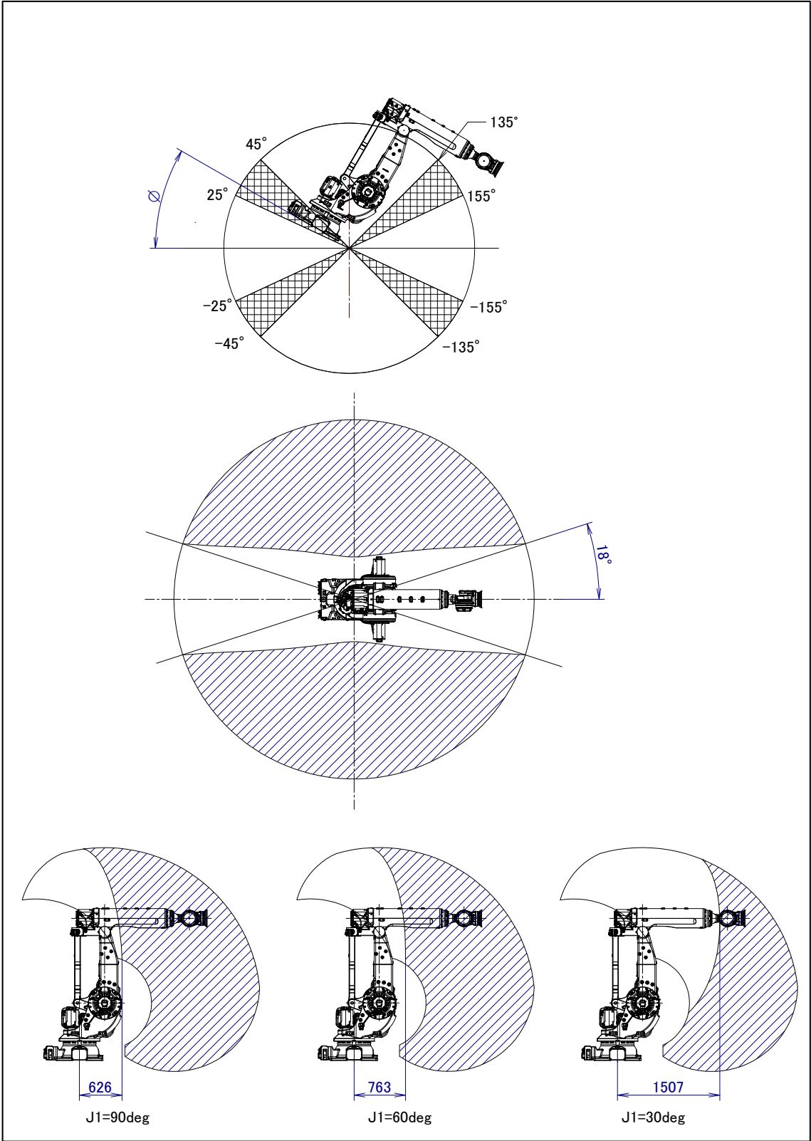
图 3.6 (I) 机器人设置角度范围(3)的动作范围 ( -155^{\circ} < \phi \leq -135^{\circ} , -45^{\circ} \leq \phi < 25^{\circ} , 25^{\circ} < \phi \leq 45^{\circ} , 135^{\circ} \leq \phi < 155^{\circ} ) (M-900iB/280)
