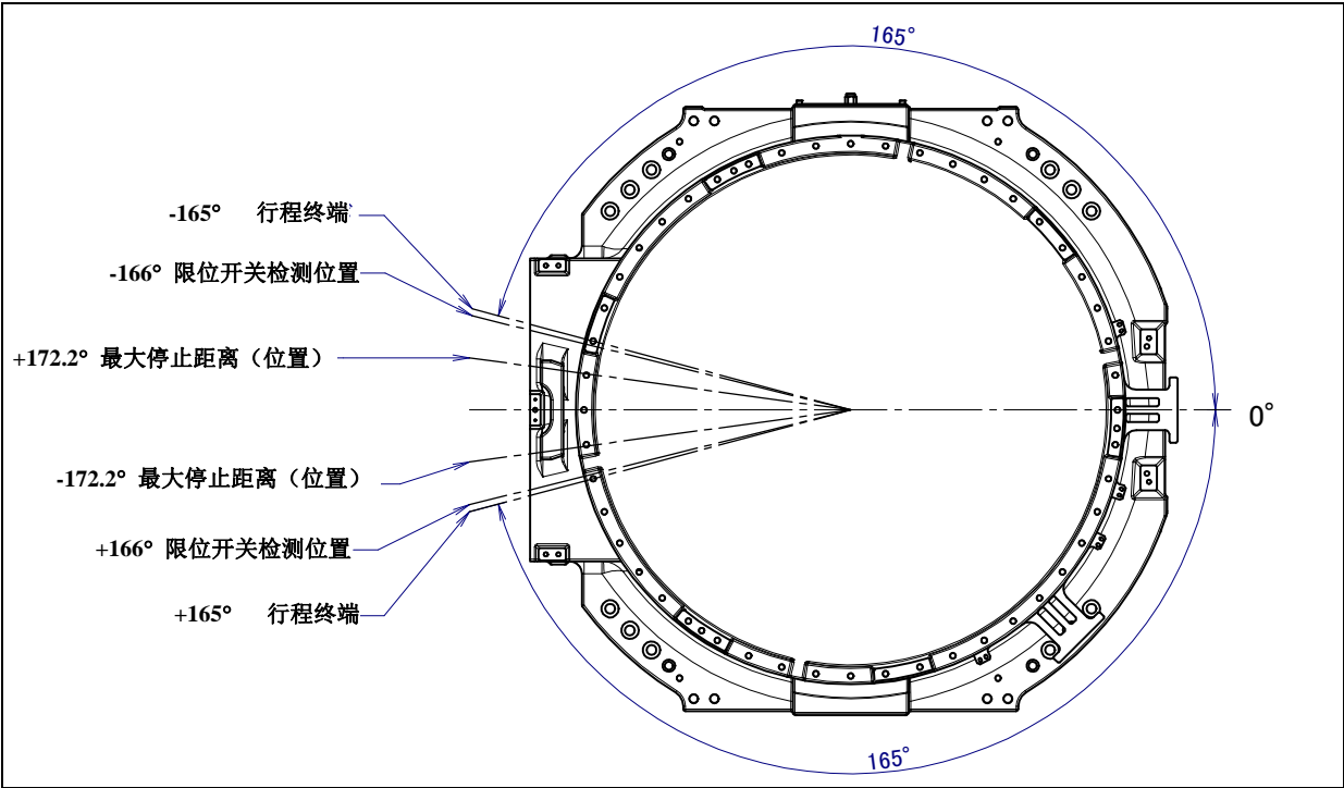
图 3.3 (c) J1 轴可动范围(M-2000iA/2300)
