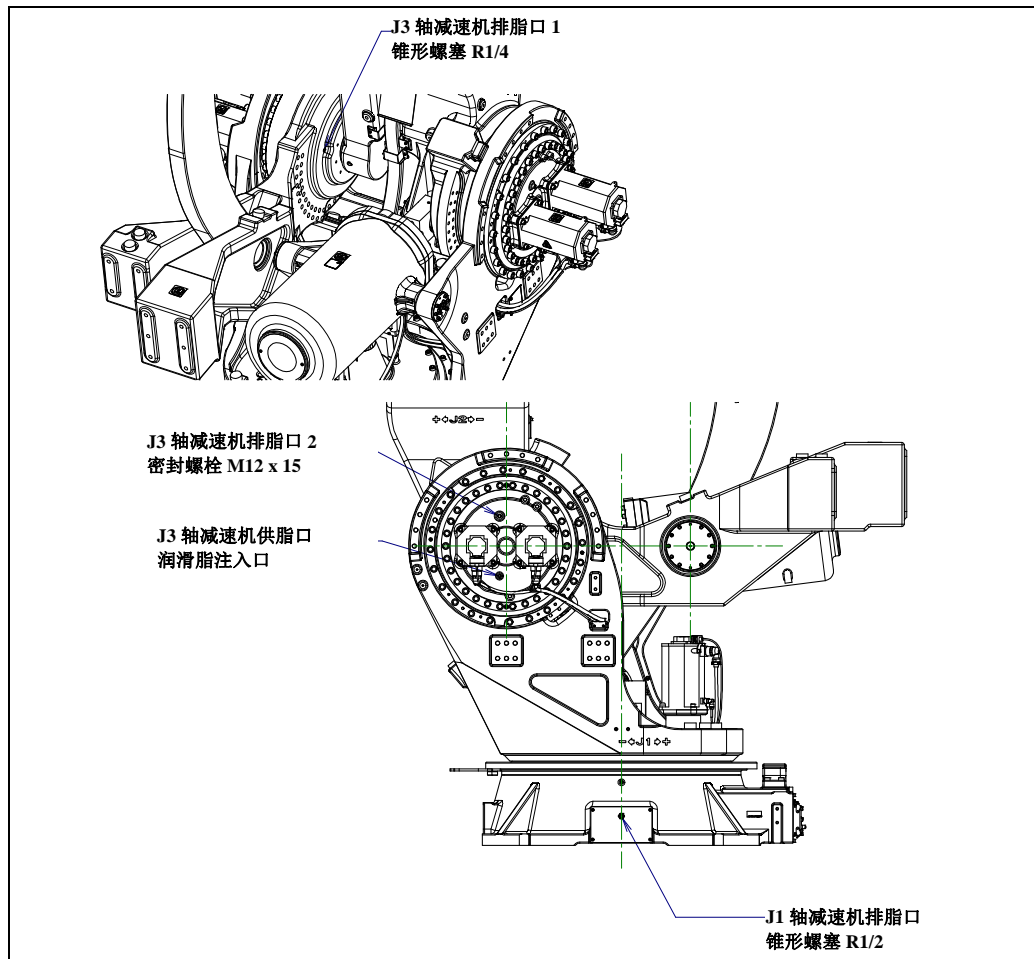
图 7.3.3 (c) J1/J2/J3 轴减速机的润滑脂的更换(M-2000iA/1200/900L) (3/3)
