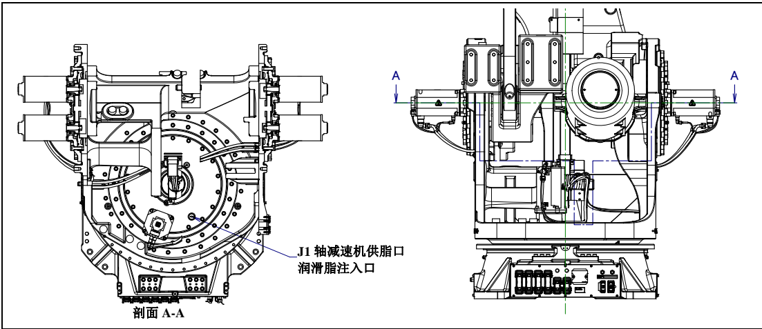
图 7.3.3 (a) J1/J2/J3 轴减速机的润滑脂的更换(M-2000iA/1200/900L) (1/3)
