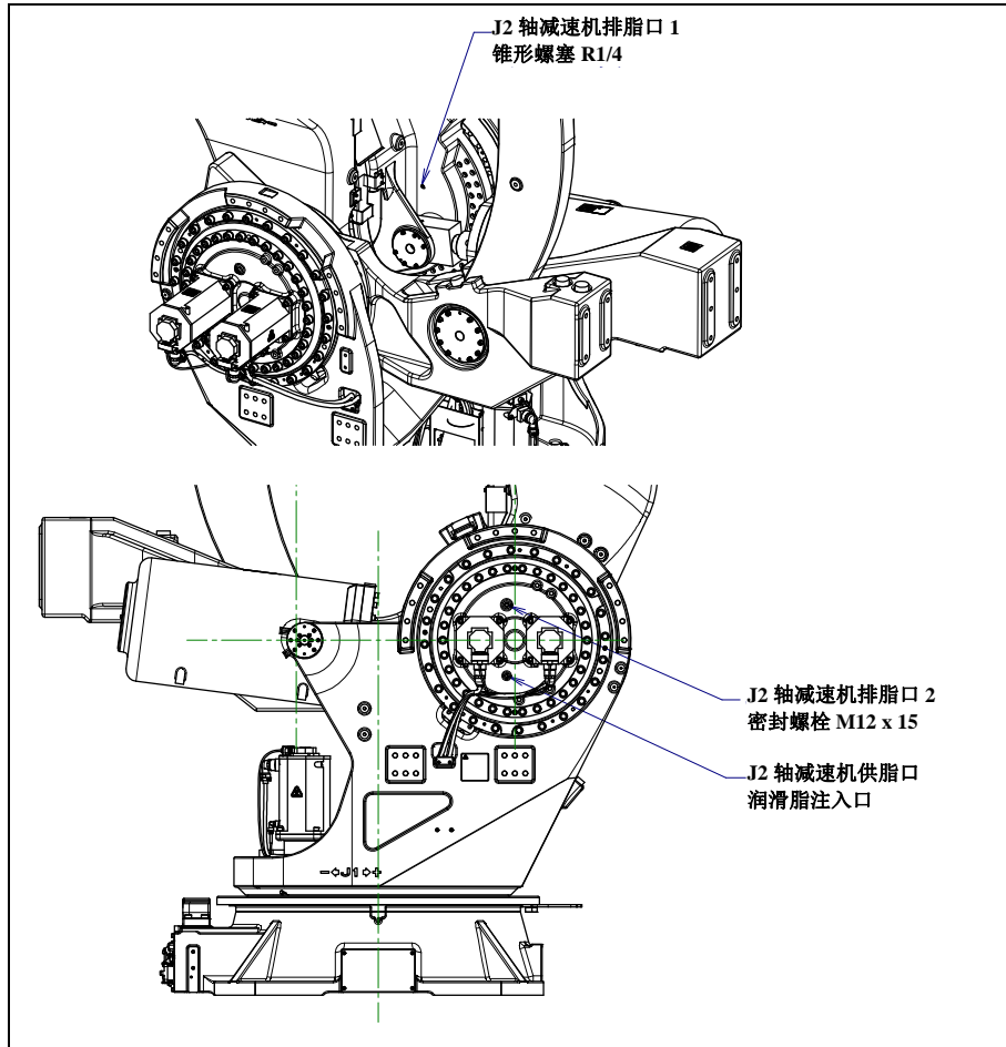
图 7.3.3 (b) J1/J2/J3 轴减速机的润滑脂的更换(M-2000iA/1200/900L) (2/3)
